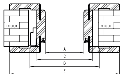
Horizontale doorsnede OF
